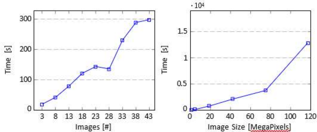
Figure 3.3: Execution times of the pipelines training phase for different image counts (left) and different image sizes(right)
